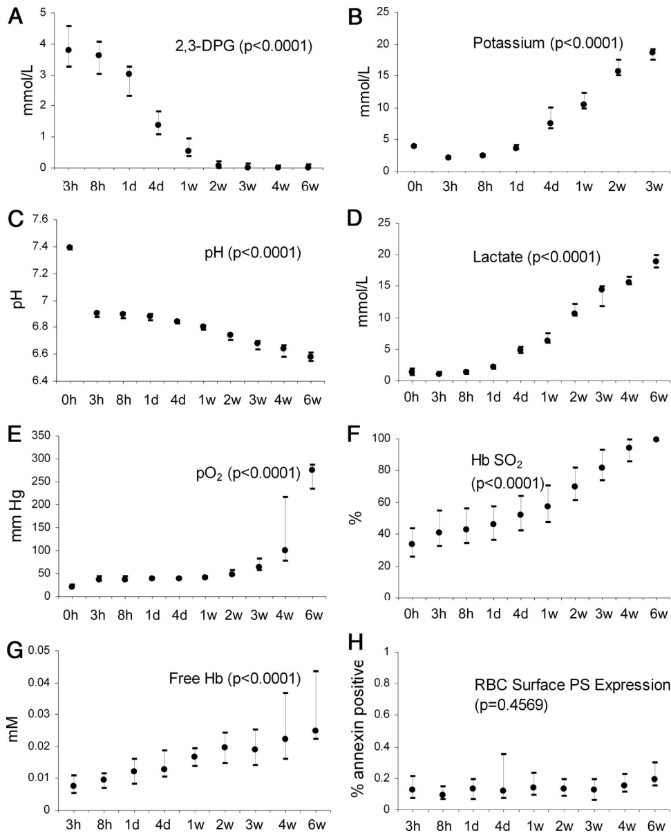
Fig. 5. Change in stored erythrocyte characteristics over time. RBC 2,3-DPG (A), potassium (B), pH (C), lactate (D), P_{O_2} (E), SO_2 (F), cell-free hemoglobin in storage medium (G), and RBC surface phosphatidyl serine (PS) expression (H) as a function of storage time. Data are median with 25th and 75th percentiles. P values represent significance for change over time. Free Hb = free hemoglobin; HbSO_2 = percent of hemoglobin saturated with oxygen; pO_2 = partial pressure of oxygen; RBC Surface PS Expression = erythrocyte surface phosphatidyl serine expression; RBC 2,3-DPG = erythrocyte 2,3-diphosphoglycerate. Reprinted from Bennett-Guerrero et al. 76 Bennett-Guerrero E, Veldman TH, Doctor A, Telen MJ, Ortel TL, Reid TS, Mulherin MA, Zhu H, Buck RD, Califf RM, McMahon TJ: Evolution of adverse changes in stored RBCs. Proc Natl Acad Sci 2007; 104:17063–8. Copyright 2007 National Academy of Sciences, U.S.A.
